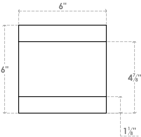
FRONT PROFILE
